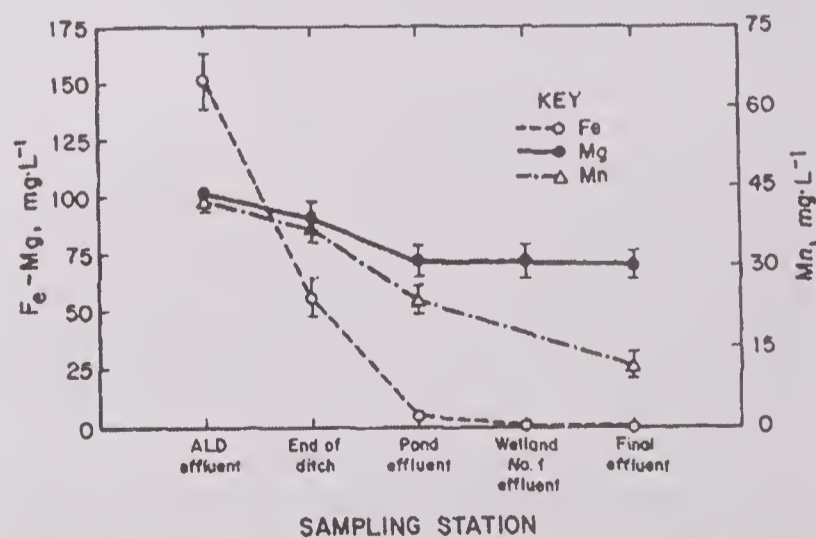
Figure 5.—Mean concentrations of Fe, Mn, and Mg at the Morrison Wetland. Mine water flows linearly from station 1 to station 5. Vertical bars are one standard error of the mean.
